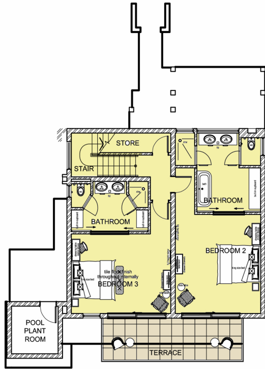
MOUNTAIN VILLA - 3 BEDROOM (Steep Slope) LOWER LEVEL PLAN
