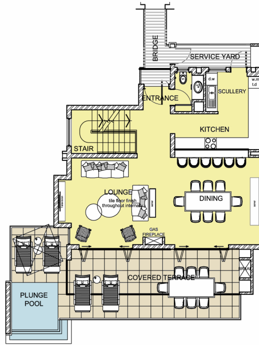
ENTRANCE LEVEL PLAN
