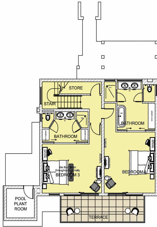
MOUNTAIN VILLA - 4 BEDROOM (Steep Slope) LOWER LEVEL PLAN
