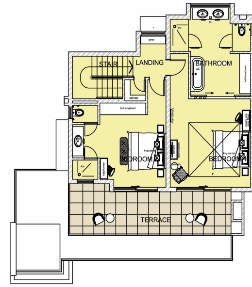
MOUNTAIN VILLA - 4 BEDROOM (Steep Slope) UPPER LEVEL PLAN
