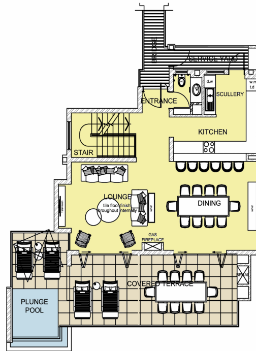
MOUNTAIN VILLA - 4 BEDROOM (Steep Slope) ENTRANCE LEVEL PLAN
