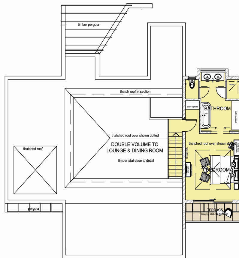
VALLEY VILLA - 3 BEDROOM (Alt 2) FIRST FLOOR PLAN
